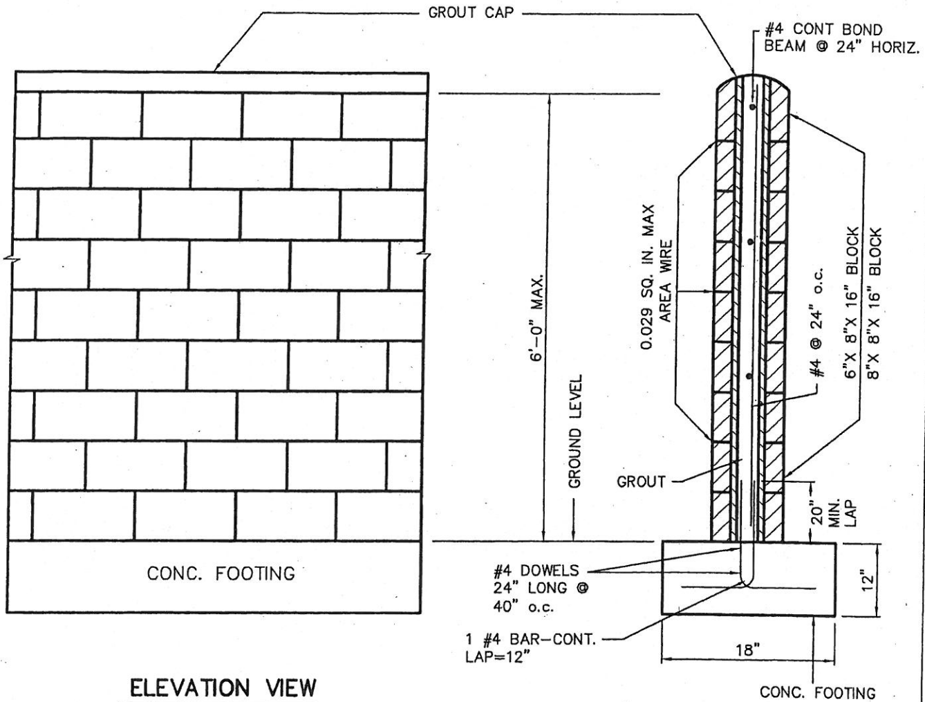
WALL SECTION
